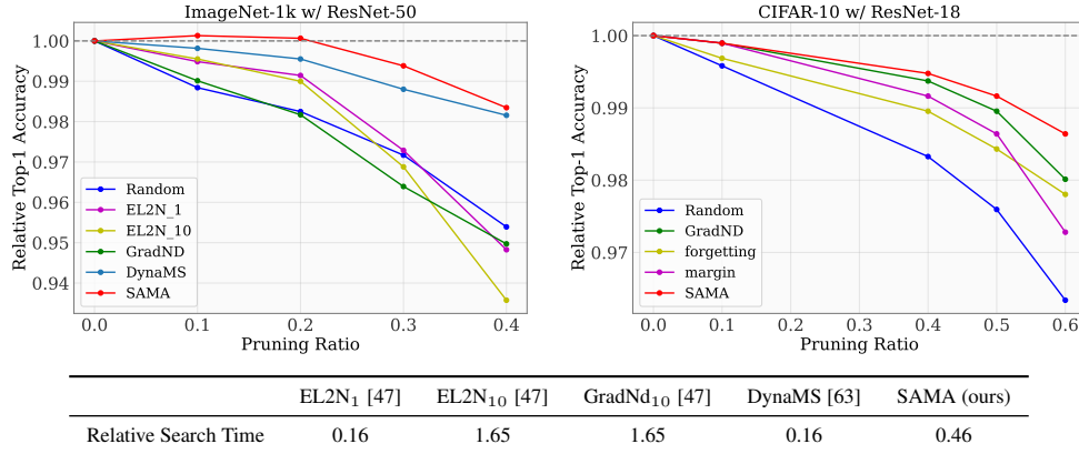
Figure 3: Top Left: ImageNet-1k data pruning results with ResNet-50. Reported numbers are relative accuracy compared to full training accuracy ( i.e. , pruned_acc/full_acc ). Accuracy for other baseline methods is obtained from DynaMS [63]. Top Right: CIFAR-10 data pruning results with ResNet-18. Accuracy for other baseline methods is obtained from Deepcore [22]. Bottom: Relative time spent in finding data to prune compared to full ImageNet-1k training time.
